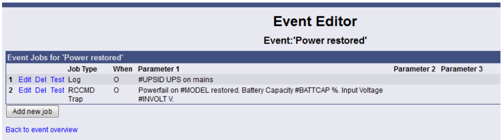
Abbildung 52: HTTP - Job Editor: RCCMD Trap Job, Event "Power restored"
