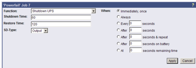
Abbildung 69: HTTP - Job Editor: Shutdown UPS-Job
