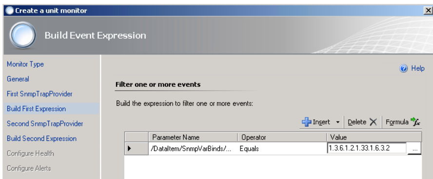
Abbildung 158: Build Event Expression Fenster
