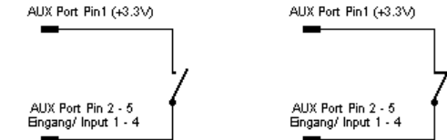
Abbildung 142: Example (Inputs): Opener or closer contact (only on hardware model CS121)
