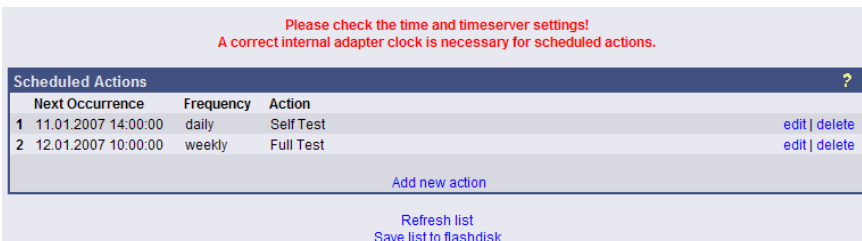
Abbildung 71: HTTP - Scheduled Actions USV Test
